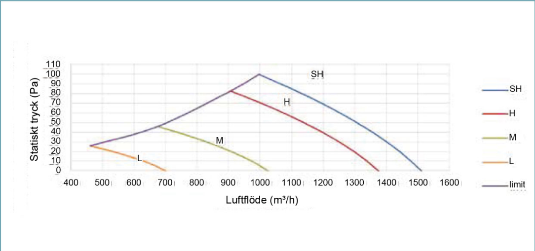
ADGH71MH
