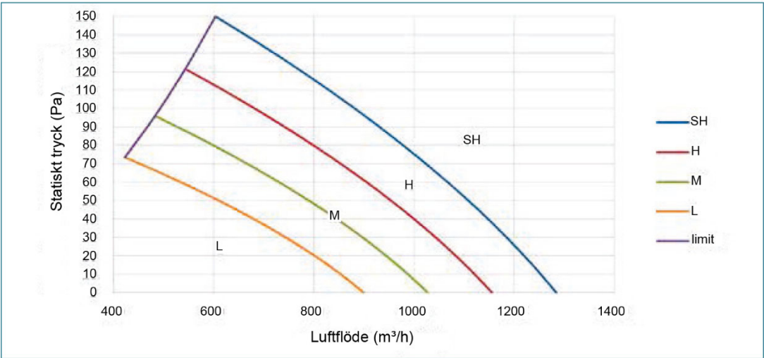
ADGH28MH
